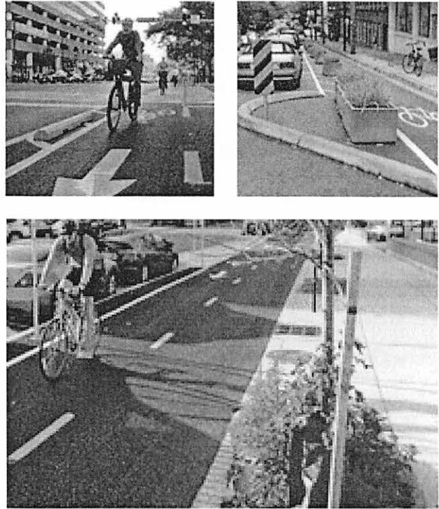
Figure 1.49: Protected bike lanes (Kirkland Design Guidelines).
