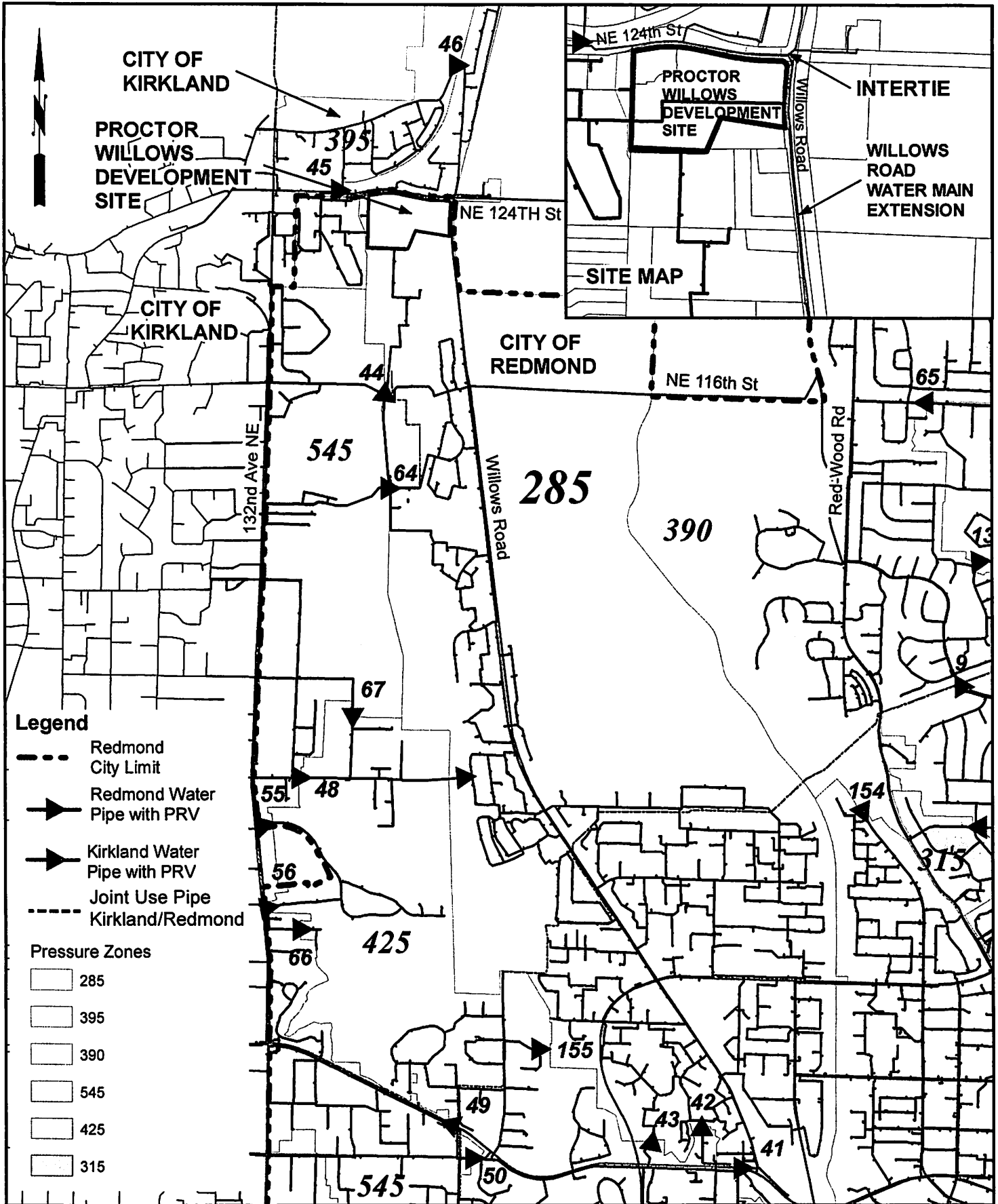
Exhibit A 285 Pressure Zone Map
