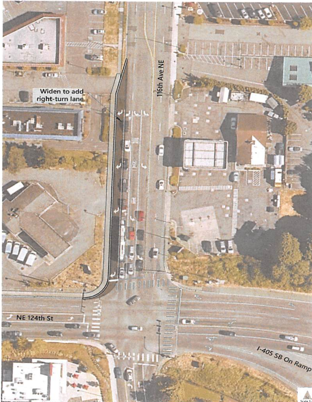
Source: Fehr & Peers, 2018 Conceptual - Not for construction. Detailed analysis and engineering required
