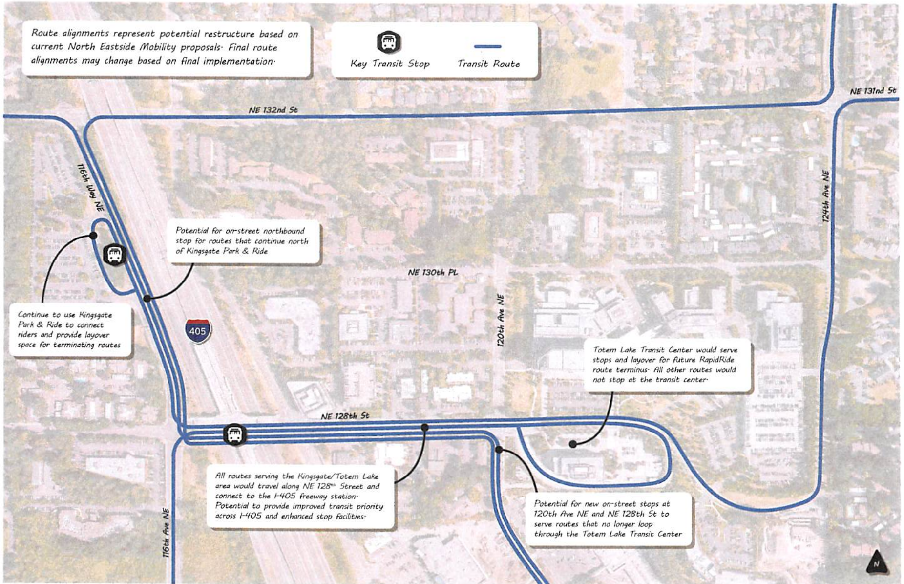
Source: Fehr & Peers, 2018 Conceptual - Not for construction. Detailed analysis and engineering required
